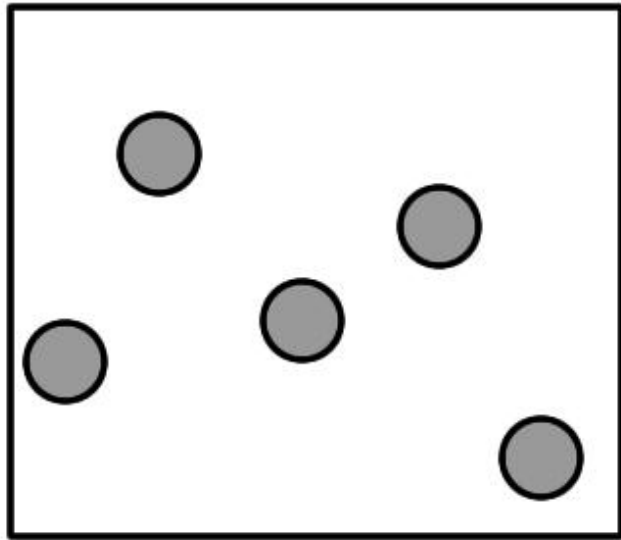
Gas
