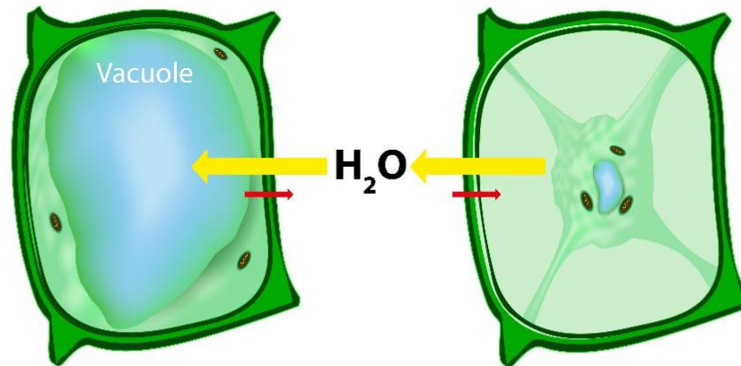
Hypotonic
