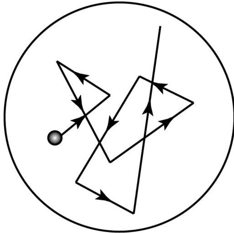
Brownian Motion
