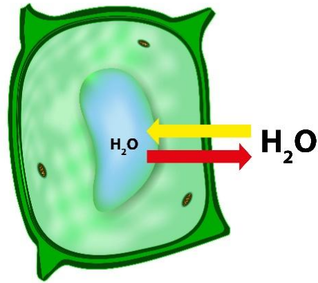
Isotonic
